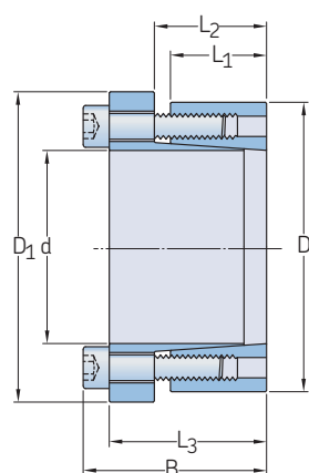
FX50, FX51
